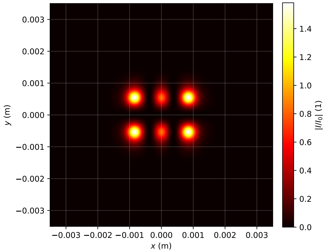
Intensity profile I(x, y, z = 0.637)/I_0 , P_{in}=3.0P_{cr} , artificial time
